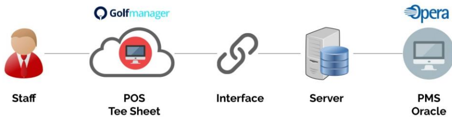
Figure 1. Architecture diagram
